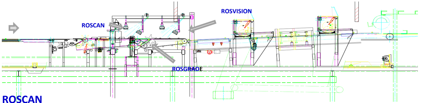
ROSCAN GRADING & OPTIMIZATION SCANNING WANE & PROFILE DETECTION
